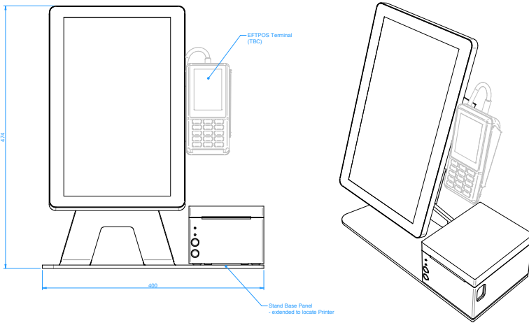
Option 3: Extended base plate to accommodate thermal printer + EFTPOS* bracket
