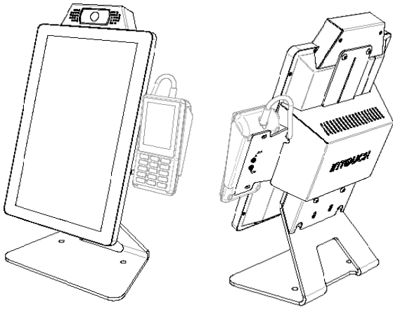
Option 1: Standard base plate + EFTPOS* bracket + fixed or tilt adjustable HD Camera
